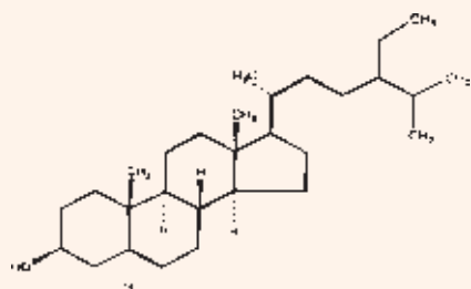
Fig. 4. Phytosterol structure
